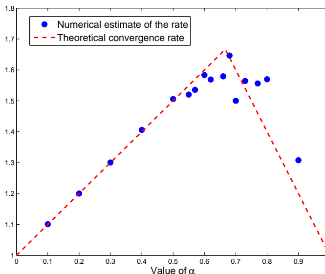
Figure 11: Predicted and estimated convergence rate with respect to \alpha .
