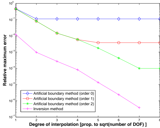
Figure 6: Comparison inversion method / absorbing boundary condition.
