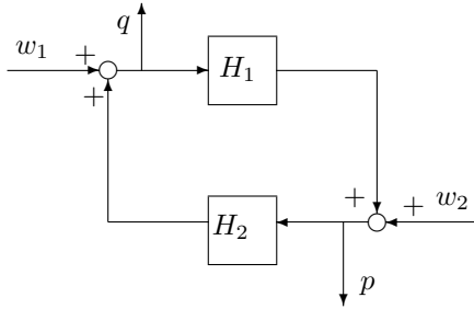
Figure 1: Internal stability
