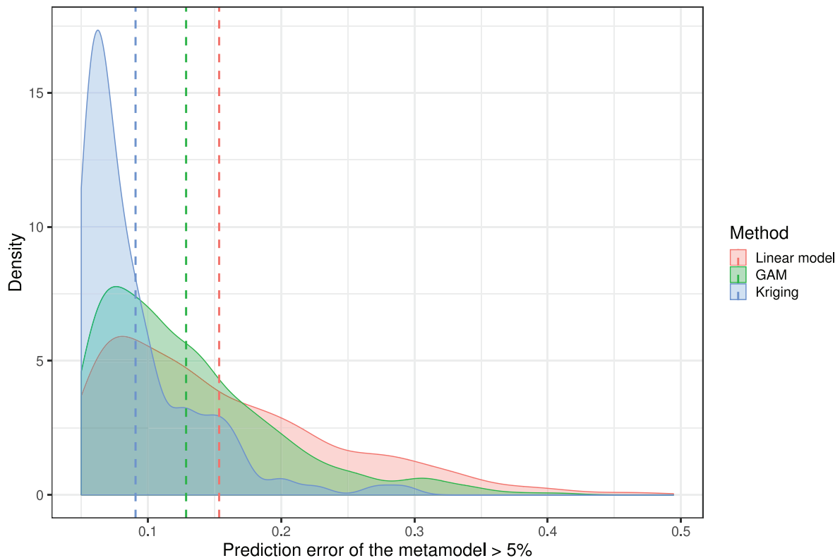
Fig. 4. Densities of the errors (larger than 5%) of the metamodel computed for the test set for the 3 different methods: linear model, GAM and kriging. Errors are defined as the difference between RDR simulated by the model and RDR predicted by the metamodel. The dotted lines represent the mean error for the corresponding metamodel.
