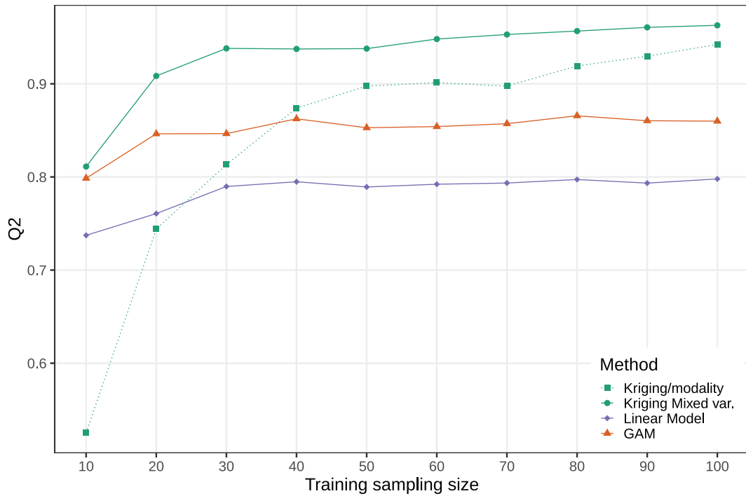
Fig. 5. Effect of training sampling size on metamodel quality with 3 different methods: linear model, GAM, and kriging (mixed and per level). The evaluation criterion is Q2 (NSE) on the test sample. For each case, the total number of points in the sample is the size defined in the x-label multiplied by 24 (pairs of levels).
