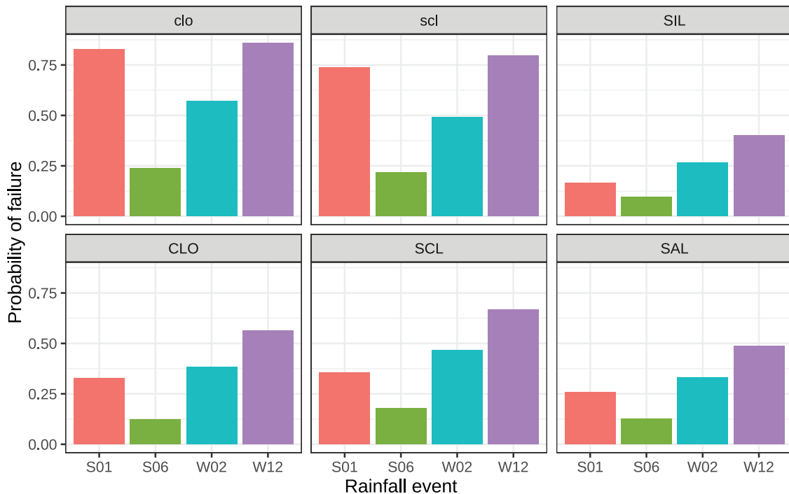
Fig. 7. Probability of failure by applying the 10 m long rule for any vegetative filter strip, for different soil and rainfall types.
