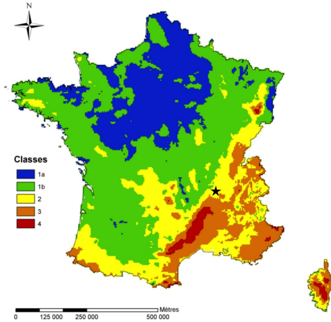
Fig. 2. Mapping of the five climate classes over France, following the upward hierarchical classification from [6]. The black star indicates the case study region, close to Lyon (Yzeron catchment).
