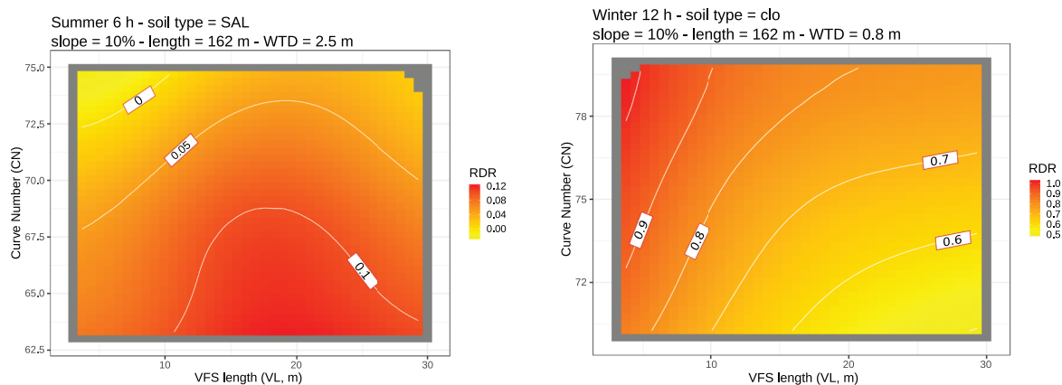
Fig. 8. RDR predicted by the metamodel considering fixed slope, length of the field, and water table depth. Left panel: VFS soil type is sandy loam soil (SAL), CN is sampled in the range [63 – 75]. Right panel: VFS soil type is newly implanted clay loam soil (clo), CN is sampled in the range [70 – 80].
