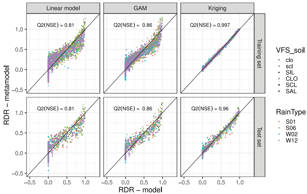
Fig. 3. Comparison between RDR from the model and from the metamodel built on the training set, accounting for qualitative inputs (6 VFS soils and 4 rainfall types) with 3 different methods: linear model, generalized additive model (GAM), and kriging (with a cov-quali-product covariance function). The predicted RDR vs the observed RDR is compared on the training set (top panels) and on the test set (bottom panels).
