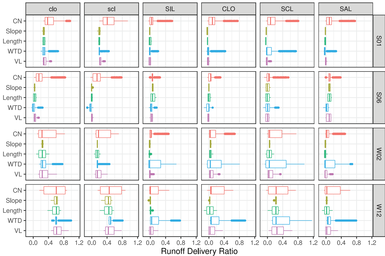
Fig. 6. Effect of quantitative input uncertainty on the RDR, depending on the qualitative input levels (6 VFS soils and 4 rainfall types - see Tables 1 and 2). The plotted distributions are obtained by predicting kriging estimated from the 100-point maximin LHS (the total number of training points is 24*100) with the cov-quali-isotropic covariance function.
